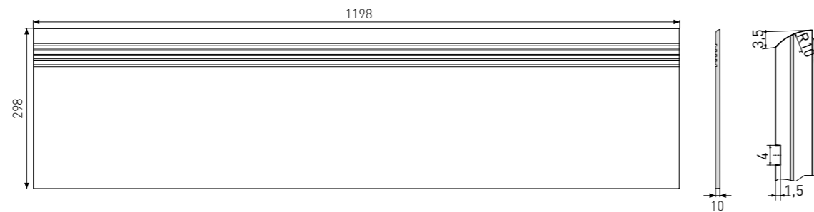
schodovka | DCPVF... | 298×1198×10 mm step tile | DCPVF... | 298×1198×10 mm
